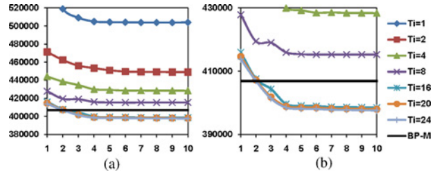
Fig. 4. (a) Energies of stereo matching on Tsukuba using tile-based BP with different number of inner iterations. (b) Close-up of the left chart. The x -axis is the index of the outer iteration and the bold horizontal line is the reference energy obtained using BP-M with 500 iterations. The energy terms are defined according to [33].
