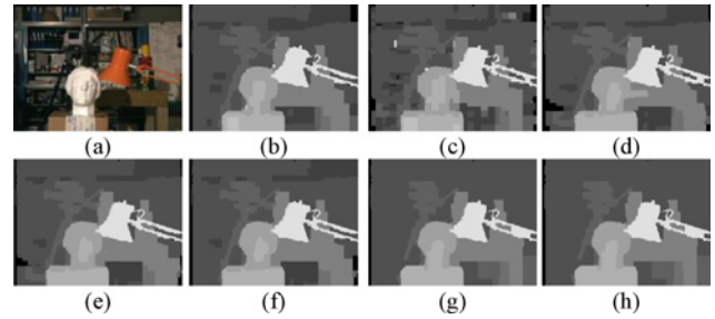
Fig. 7. Stereo matching of Tsukuba . (a) Left image. (b) Result of BP-M after 500 iterations. (c) Result of block-based BP. (d) Result of tile-based BP without inverse raster scan. (e) Result of tile-based BP with one outer iteration. (f) Twenty outer iterations. (g) Result of TRW-S. (h) Ground truth.
