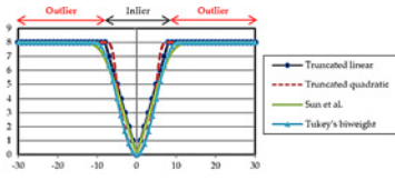
Fig. 10. Illustration of several typical robust functions. We choose the parameters to match the cut-off regions and the penalty value of the outlier of different functions.
