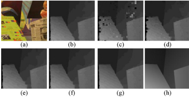
Fig. 8. Stereo matching of Venus . (a) Left image. (b) Result of BP-M after 500 iterations. (c) Result of block-based BP. (d) Result of tile-based BP without inverse raster scan. (e) Result of tile-based BP with one outer iteration. (f) Twenty outer iterations. (g) Result of TRW-S. (h) Ground truth.
