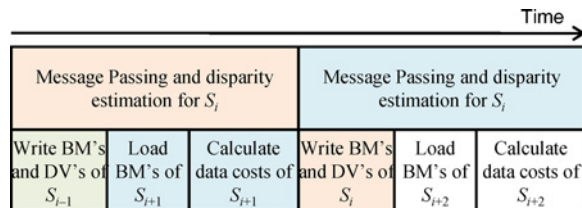
Fig. 15. Two-stage pipeline in the VLSI circuit. Here BM denotes boundary message and DV denotes disparity value.
