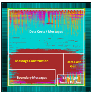
Fig. 13. Floorplan of the developed VLSI circuit.
