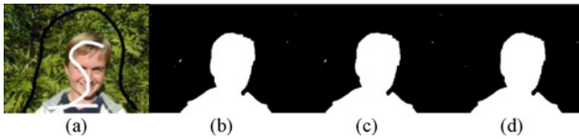
Fig. 5. Binary image segmentation of the benchmark Person . (a) Input image and the strokes. (b) Result of BP-M. (c) Result of tile-based BP. (d) Result of TRW-S.
