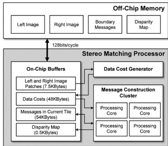
Fig. 12. Systematic overview of the developed VLSI circuit.
