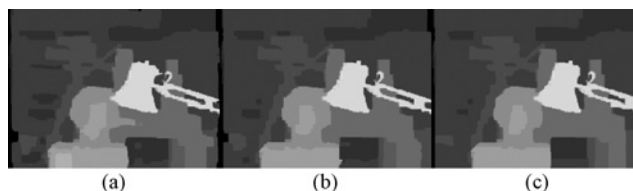
Fig. 16. Disparity maps of the dataset Tsukuba by the hardware implementation using different numbers of iterations. (a) (T_I, T_O) = (3, 1) . (b) (T_I, T_O) = (20, 1) . (c) (T_I, T_O) = (20, 5) .
