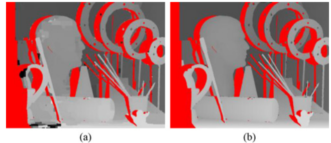
Fig. 9. Stereo matching of a high-resolution dataset Art . The image size ( N ) is 1390-by-1110 and the disparity range ( L ) is 240. (a) Result of tile-based BP with (B, T_I, T_O) = (16, 20, 12) . (b) Ground truth. For better visualization, the occluded regions which are not handled by the adopted simple energy functions are masked as red.
