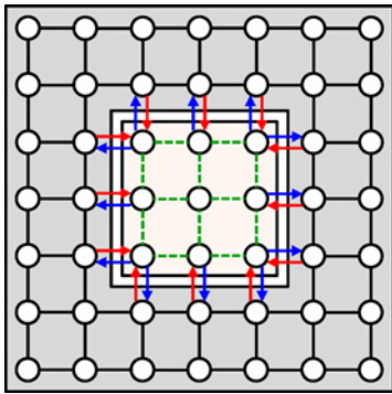
Fig. 2. 7-by-7 MRF is split into two subsets. One subset N_1 contains the nodes in the tile (the light-shaded region) and the other subset N_2 contains all other nodes (the dark-shaded region).
