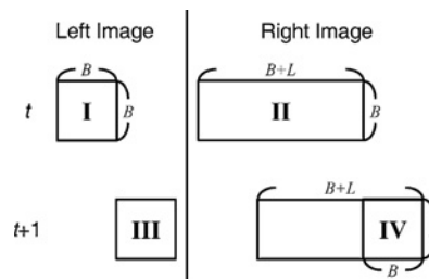
Fig. 14. Data reuse scheme for calculating the data costs. When we calculate the data costs of the first tile of a row, we need to load B^2 pixels in the left image (I) and B(B+L) pixels in the right image (II). However, in calculating the data costs of the next tile, only B^2 additional pixels are loaded (IV).
