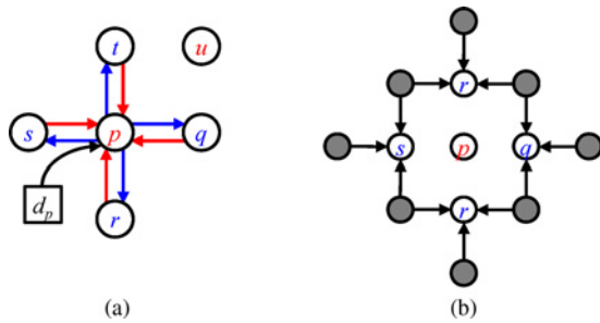
Fig. 1. (a) Message passing in the bipartite graph. To generate the messages from node p to its neighbors q , r , s , and t (outward blue arrows) we only need to access the messages toward (inward red arrows) and the data cost d_p . The messages related to node u are never involved. (b) To generate the messages toward p , we need the messages from the neighbors of p (the shaded circles).
